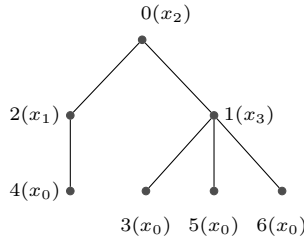
Fig. 5.2. A labeling on an increasing tree.
