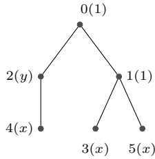
Fig. 3.1. The labeling of a 0-1-2 increasing tree on {0, 1, 2, 3, 4, 5}.
